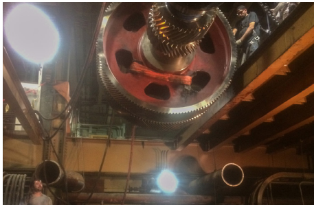
Field services gearbox rebuild at tire plant
