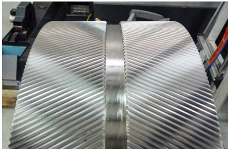
Double helical gear
