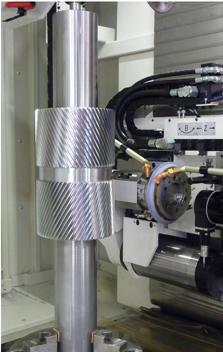
Double helical shaft being ground
