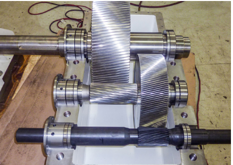
Custom dam gate gearbox, inside
