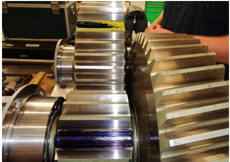
Custom straightener gearbox for steel mill, inside
